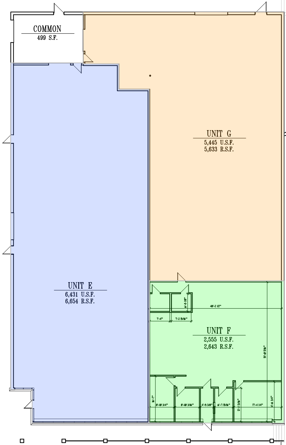
EXISTING FLOOR PLAN - 14,930 S.F. SCALE: 1/20" = 1'-0"
